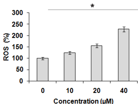
Figure 7. Effect of indicated concentrations of safranal on ROS generation. The experiments were carried out in triplicate and expressed as mean±SD (*p<0.05). The Figure shows that safranal led to the production of ROS in a concentration-dependent manner.
