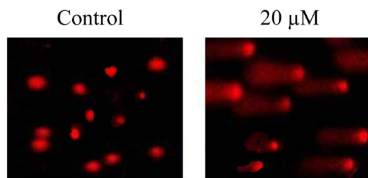
Figure 4. Comet assay showing DNA damage induced by safranal at IC_{50} (20 \mu M).
