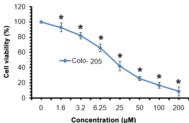
Figure 2. Effect of safranal on cell viability as determined by MTT assay. The experiments were carried out in triplicate and expressed as mean \pm SD (* p <0.05). The Figure shows that the cell viability decreased with increasing safranal concentration (dose-dependent response).
