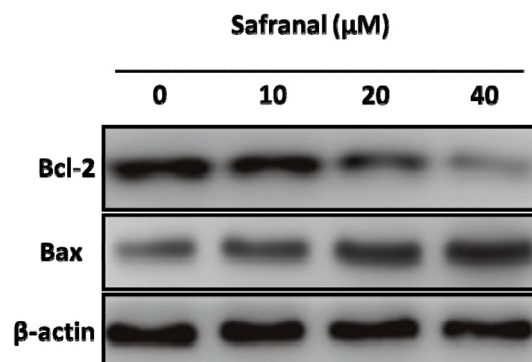
Figure 5. Estimation of apoptotic cell populations of colo205 cells after treatment with safranal at IC_{50} . The experiments were carried out in triplicate. The Figure reveals that Bax expression increased and Bcl-2 decreased in a concentration-dependent manner.
