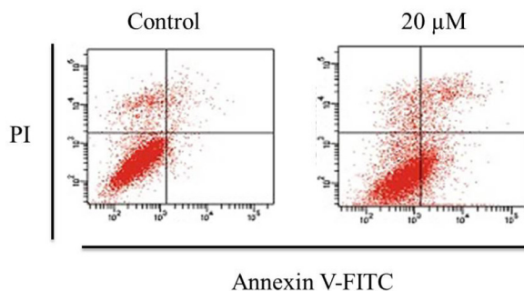
Figure 6. Annexin V/PI showing apoptotic cell populations. The experiments were carried out in triplicate. The Figure shows that safranal triggered apoptosis at IC_{50} (20 \mu M).
