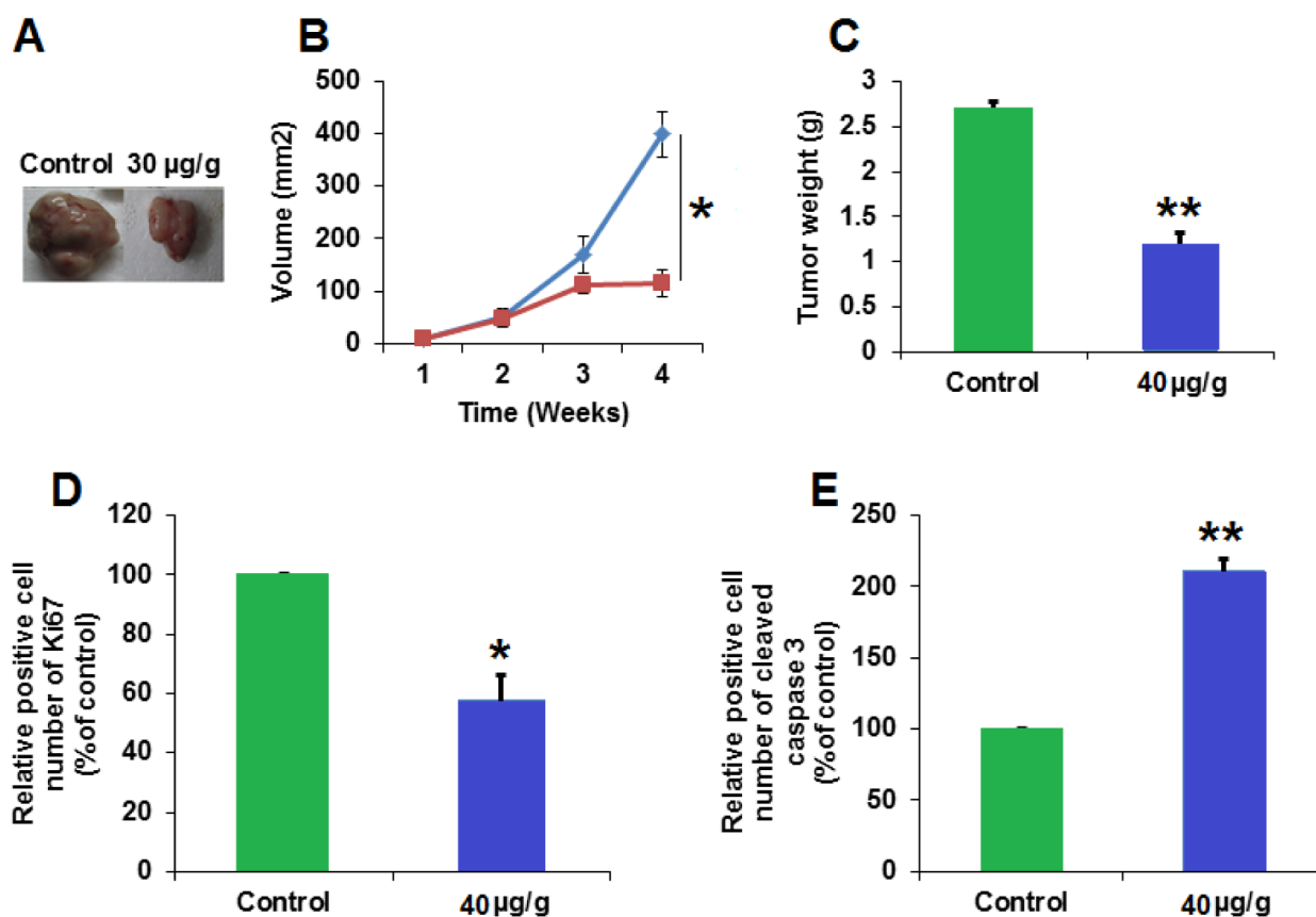
Figure 8. Argabin inhibits oral tumor growth in vivo . (A) Representative tumor-bearing nude mice and tumors isolated from the control and arglabin-treated groups. (B) Tumor volumes. (C) Tumor weights at the indicated time intervals and dosages. (D) Relative percentages of Ki67, and (E) cleaved caspase 3-positive cells. Results are shown as mean \pm standard deviation of three biological replicates. The differences were considered significant at * p < 0.01 , and ** p < 0.001 .
