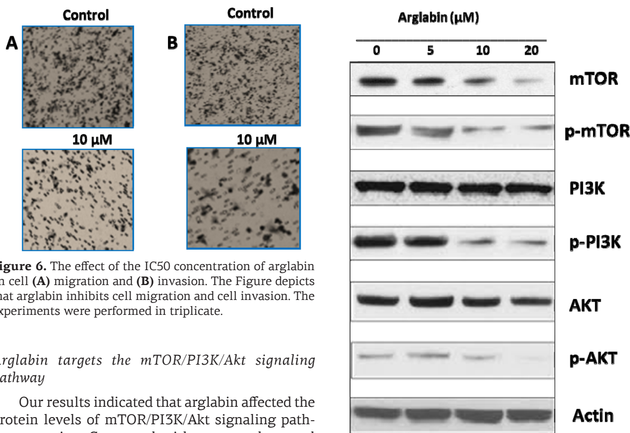
Figure 7. Western blot analysis of the levels of mTOR/PI3K/Akt pathway proteins showing that arglabin caused dose-dependent inhibition of p-mTOR, p-PI3K and p-AKT proteins. The experiments were performed in triplicate.
